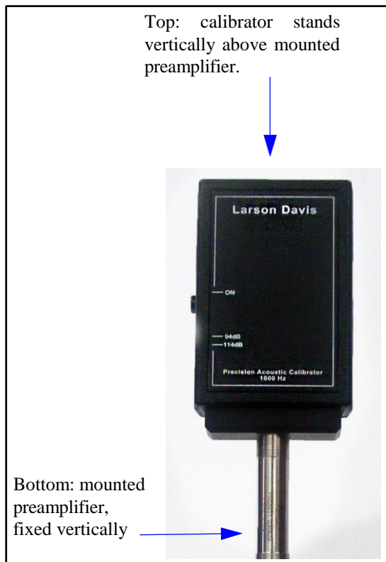
FIGURE 2-1 Vertical Positioning
