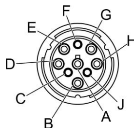
Figure 5: J1939-13 Type II CAN connector pinout.
